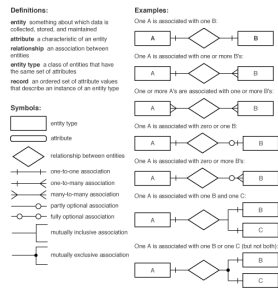
Figure 8–1 Rules for Drawing an E-R Diagram
