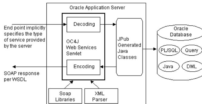
Figure 12-1 Web Services Calling In to the Database
