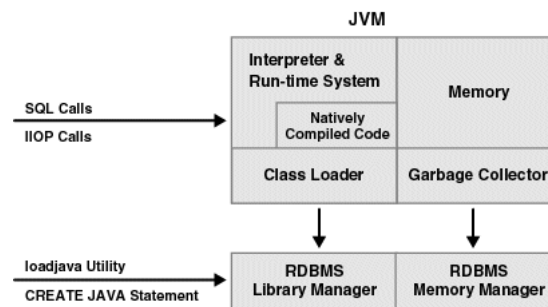
Figure 1-9 Main Components of the OracleJVM
