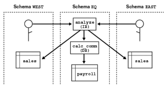
Figure 2-5 Indirect Access
