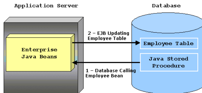
Figure 1–2 EJB Call-out
