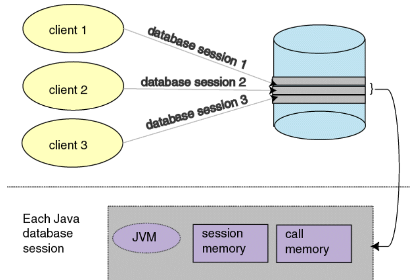
Figure 2–1 Java Environment Within Each Database Session
