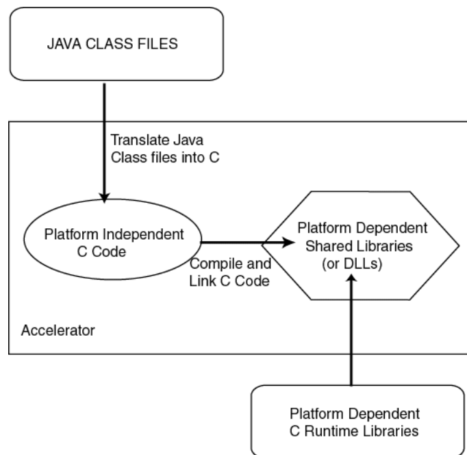
Figure 10–1 Native Compilation Using Accelerator
