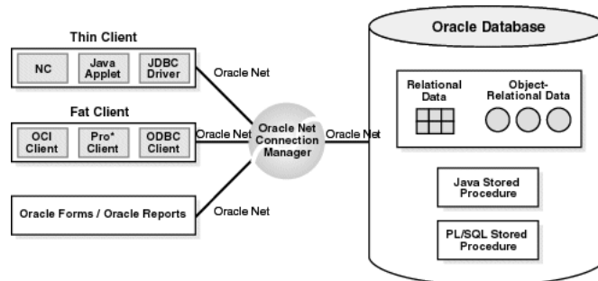
Figure 1-7 Two-Tier Client/Server Configuration
