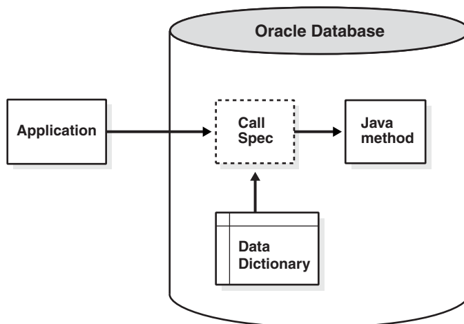
Figure 6–1 Calling a Java Method
