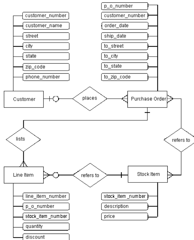
Figure 8-2 E-R Diagram for Purchase Order Application
