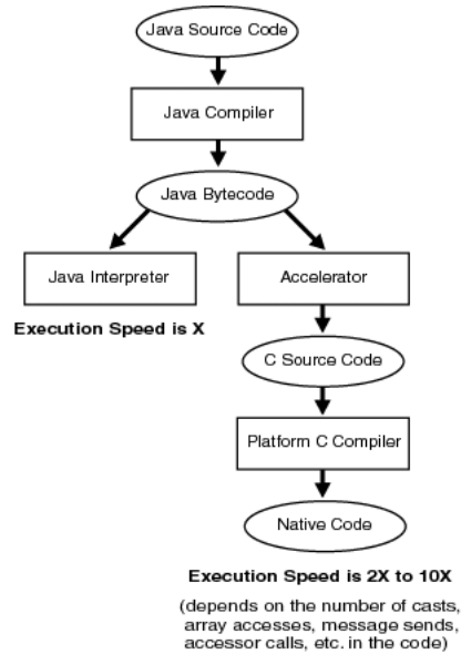
Figure 1–8 Interpreter versus Accelerator
