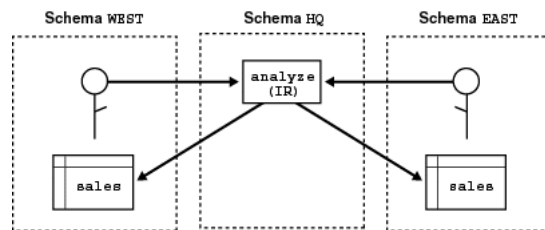
Figure 2-4 Invoker-Rights Solution
