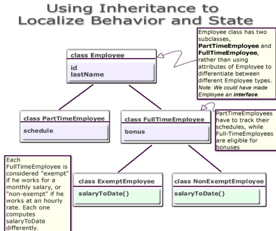
Figure 1–4 Class Hierarchy
