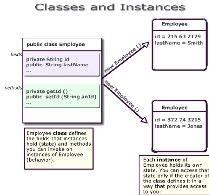
Figure 1–3 Classes and Instances
