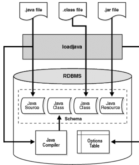
Figure 2-2 Loading Java into the Oracle Database
