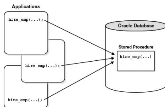
Figure 5-1 Calling a Stored Procedure
