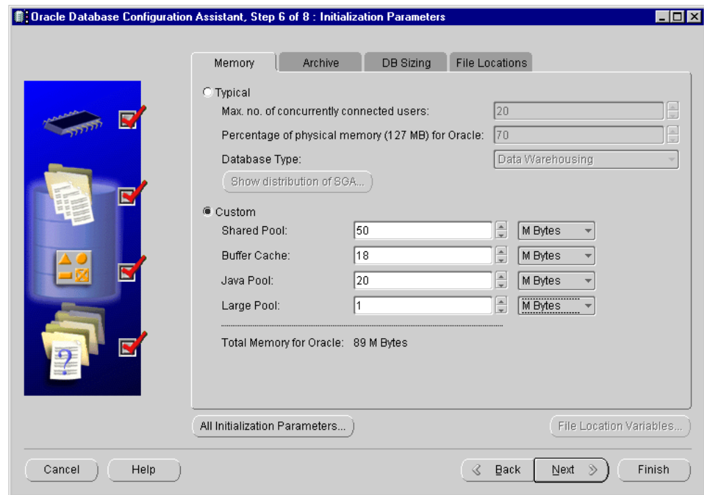
Figure 10–2 Configuring OracleJVM Memory Parameters
