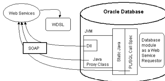
Figure 12–2 Calling Web Services From Within the Database
