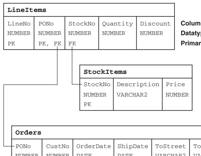
Figure 8-3 Schema Plan for Purchase Order Application
